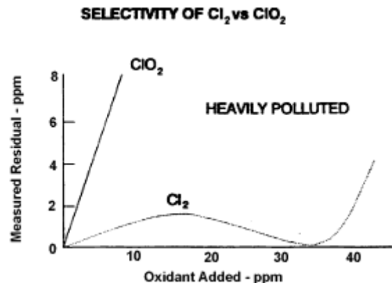
Figure 2: chlorine dioxide is more selective as an oxidizer than chlorine. While dosing the same concentrations, the residual concentration of chlorine dioxide is much higher with heavy pollution than the residual concentration of chlorine.
